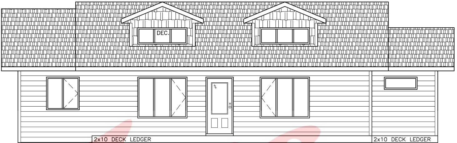
HIGHROCK FRONT ELEVATION
